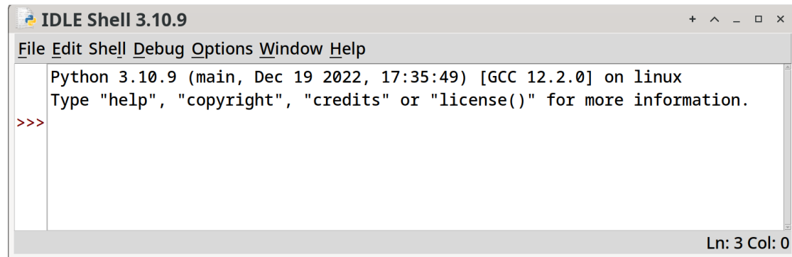
Figure 3.1: IDLE Window
